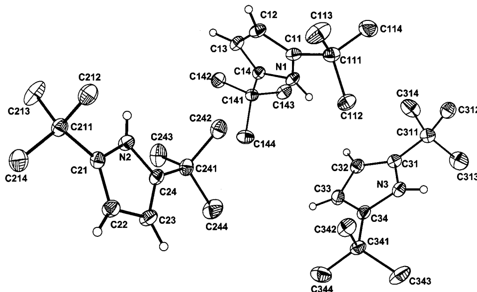
Figure 1. Molecular structure and numbering scheme of the asymmetric unit of HPyr* ( 1 ); the ellipsoids represent a probability of 40%; the hydrogen atoms of the tert -butyl groups are omitted for clarity; those of the azacyclopentadiene unit are drawn with arbitrary radii [a]
