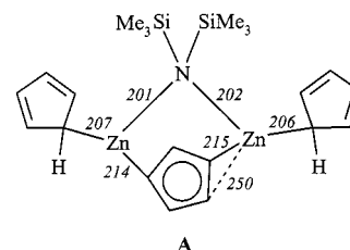
Scheme 1. Selected bond lengths [pm] in tris(cyclopentadienyl)di-zinc \mu -bis(trimethylsilyl)amide ( A )
